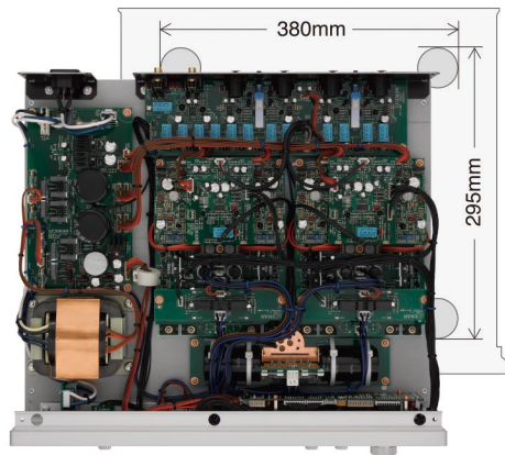
Internal configuration
