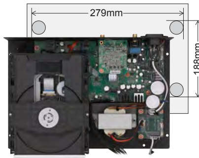
Internal configuration
