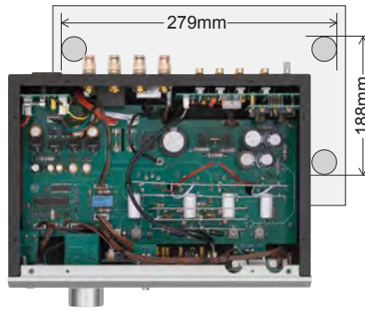
Internal configuration
