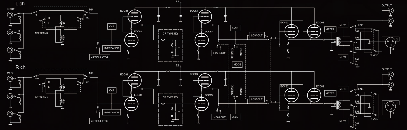
EQ-500 BLOCK DIAGRAM (AMP)
