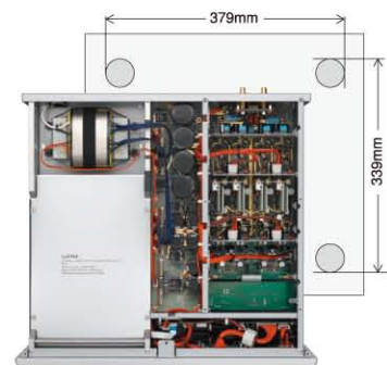
Internal configuration
